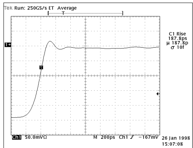
Figure 3. 17.5 ps edge with 2 GHz scope.
